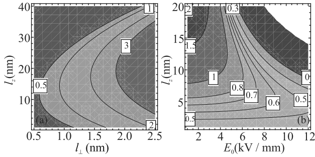
Fig. 1. (Color online) The domain formation energy \delta\mathcal{E} (in eV) versus E_0 , l_\perp , and l_z in the presence of DW conduction for the LN parameters, w_0 = 3 erg/cm 2 and w_1 = 15 erg/cm 2 . (a) – Contour lines \delta\mathcal{E}(l_\perp, l_z) = \text{const} for E_0 = 4 kV/mm. (b) – Contour lines \delta\mathcal{E}(E_0, l_z) = \text{const} for l_\perp = 1 nm
